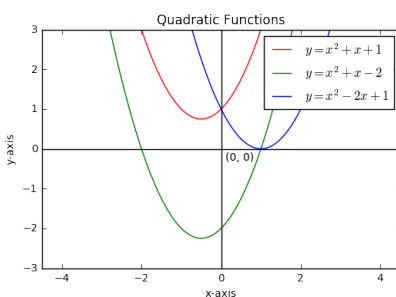
Figure 1: Quadratic Functions
